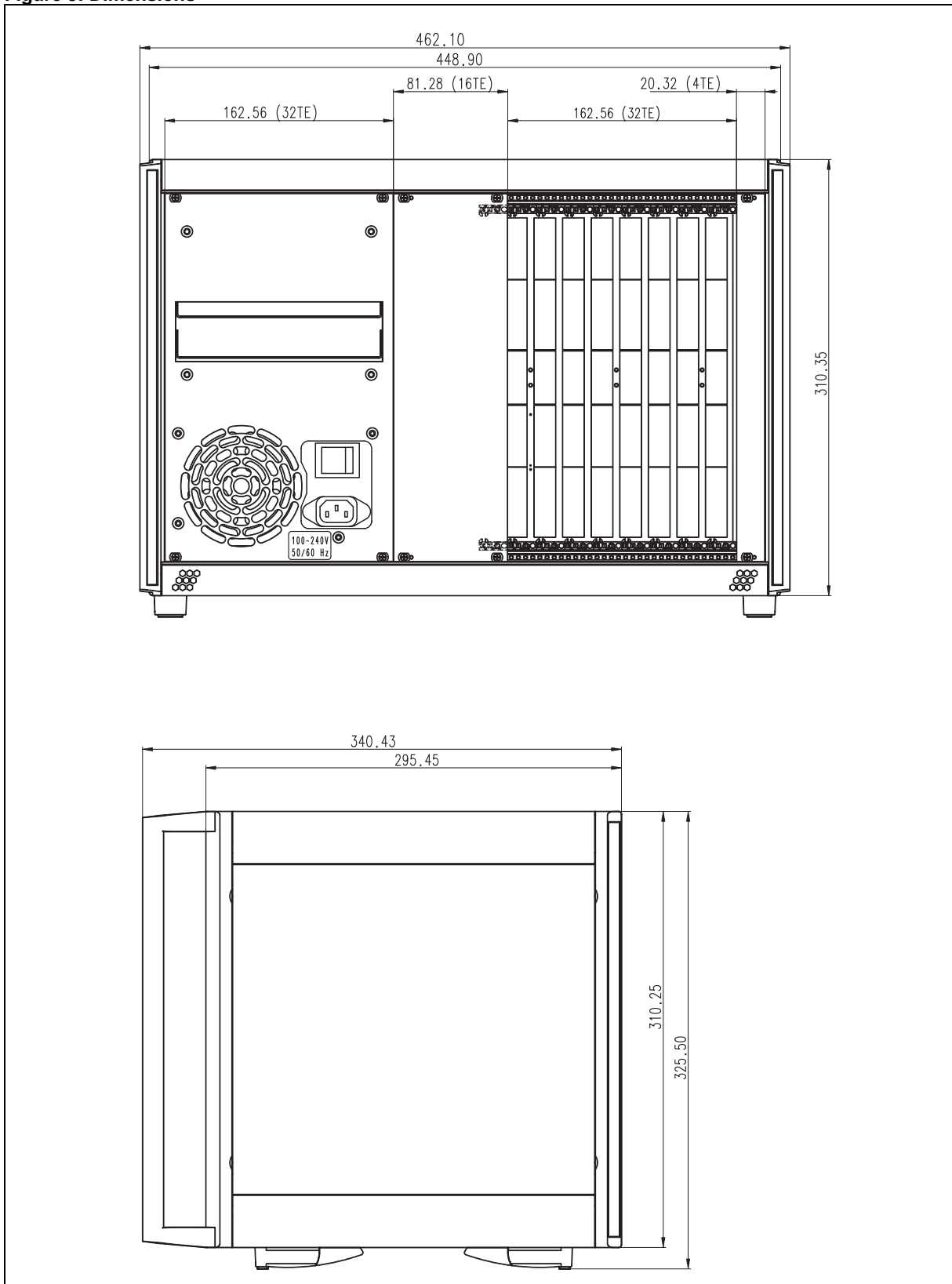
Figure 3: Dimensions
